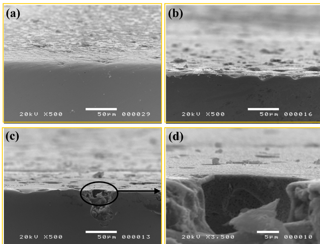
Fig. 9. SEM micrographs for the \text{Al}_x\text{CrFe}_{1.5}\text{MnNi}_{0.5} alloys with aluminium content (a) x=0 , (b) x=0.3 mol, (c) x=0.5 mol, (d) higher magnification of micrograph 9(c) after anodic polarization exceeded the breakdown potential ( >1.25 V_{\text{SHE}} ) in 0.5 M \text{H}_2\text{SO}_4 .
