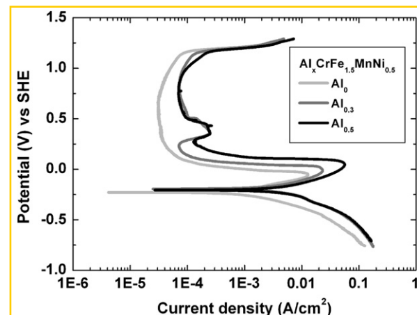
Fig. 1. The effect of aluminium on the potentiodynamic polarization curves of the \text{Al}_x\text{CrFe}_{1.5}\text{MnNi}_{0.5} ( x = 0, 0.3, 0.5 ) alloys in 0.5\text{ M H}_2\text{SO}_4 solution.
