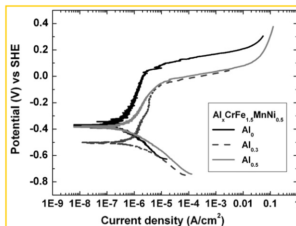
Fig. 3. Comparisons of the potentiodynamic polarization curves for the \text{Al}_x\text{CrFe}_{1.5}\text{MnNi}_{0.5} ( x = 0, 0.3, 0.5 ) alloys in 1 M NaCl solution
