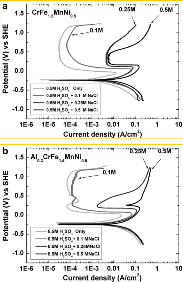
Fig. 4. Potentiodynamic polarization curves for (a) \text{CrFe}_{1.5}\text{MnNi}_{0.5} and (b) \text{Al}_{0.3}\text{CrFe}_{1.5}\text{MnNi}_{0.5} alloys obtained in 0.5 M \text{H}_2\text{SO}_4/\text{x} M NaCl ( \text{x} = 0\text{--}0.5 M) solutions.
