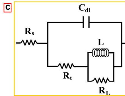
Fig. 7. The (a) Nyquist and (b) Bode plots and (c) the equivalent electrical circuit representative of the electrode interface for the \text{CrFe}_{1.5}\text{MnNi}_{0.5} alloy in 0.5 M \text{H}_2\text{SO}_4 solution. Scattered points are the experimental data and solid lines show the model fit.
